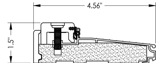
38 INSWING THRESHOLD Inswing Composite Adjustable Sill
