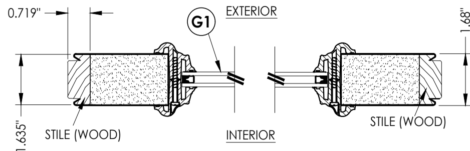
1 HORIZONTAL CROSS SECTION 3
